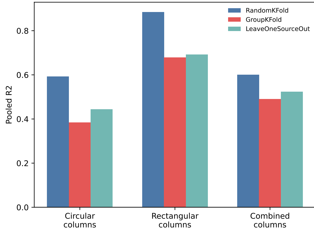
DesignSafe RC column lateral-strength validation
