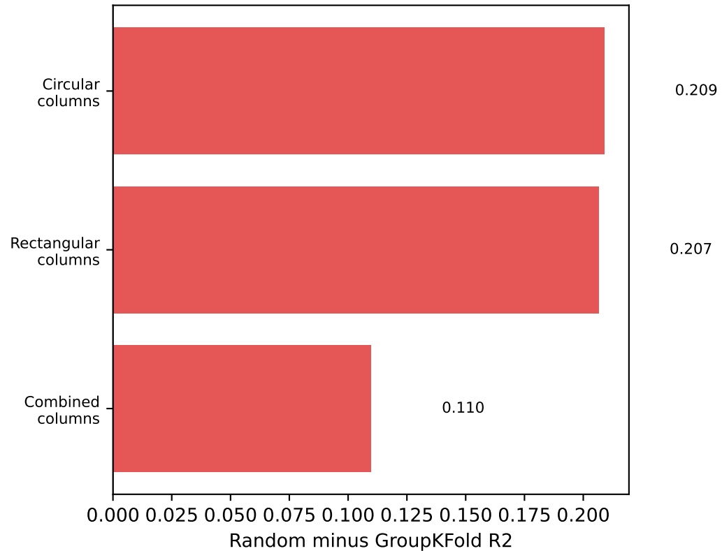
Validation gap
